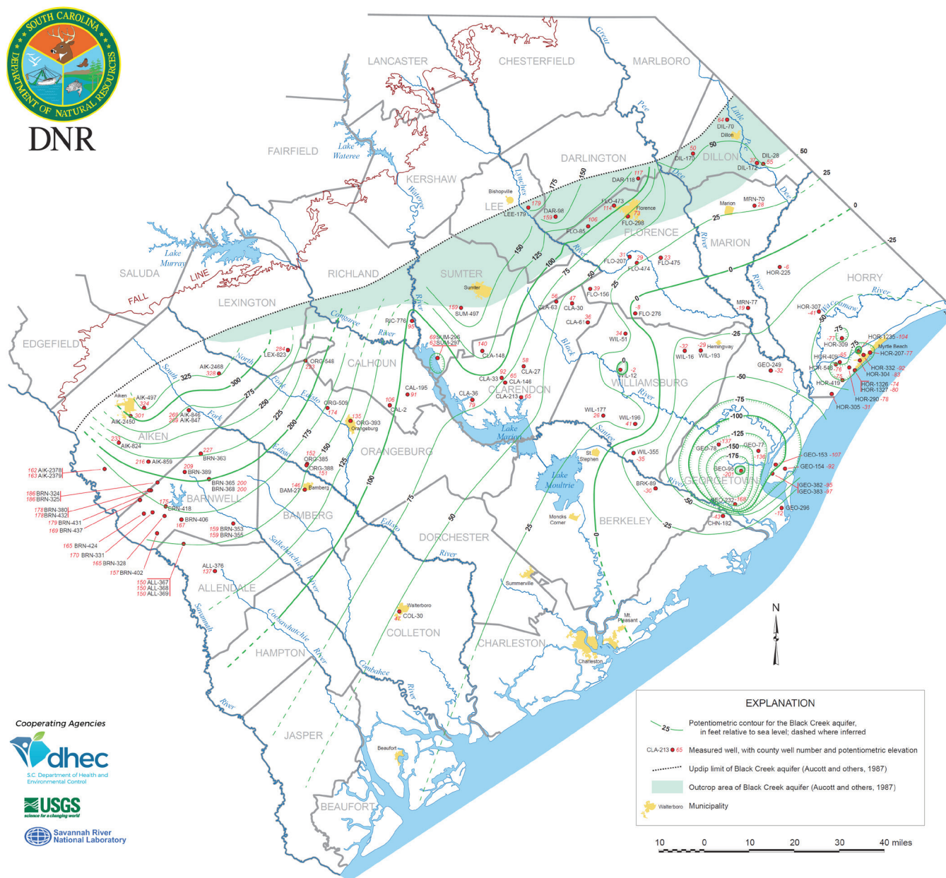
Figure 14: Black Creek/Crouch Branch aquifer potentiometric map (Wachob & Czwartacki, 2016).
